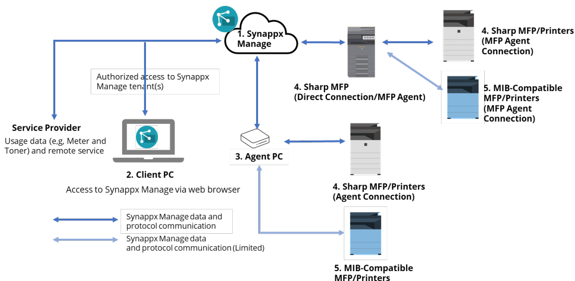
Synappx Manage MFP/Printer Monitoring Diagram
