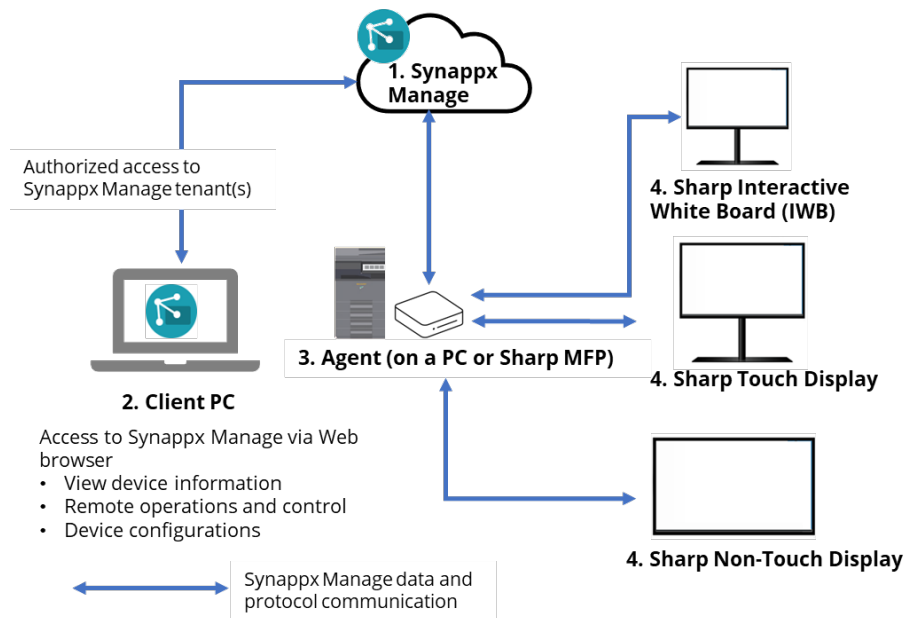
Synappx Manage Display Monitoring Diagram
